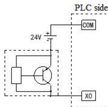
2-wire (NPN type) proximity switch wiring diagram
