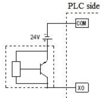
3-wire (PNP type) proximity switch wiring diagram
