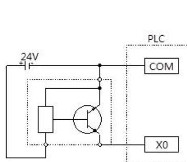
3-wire (NPN type) proximity switch wiring diagram
