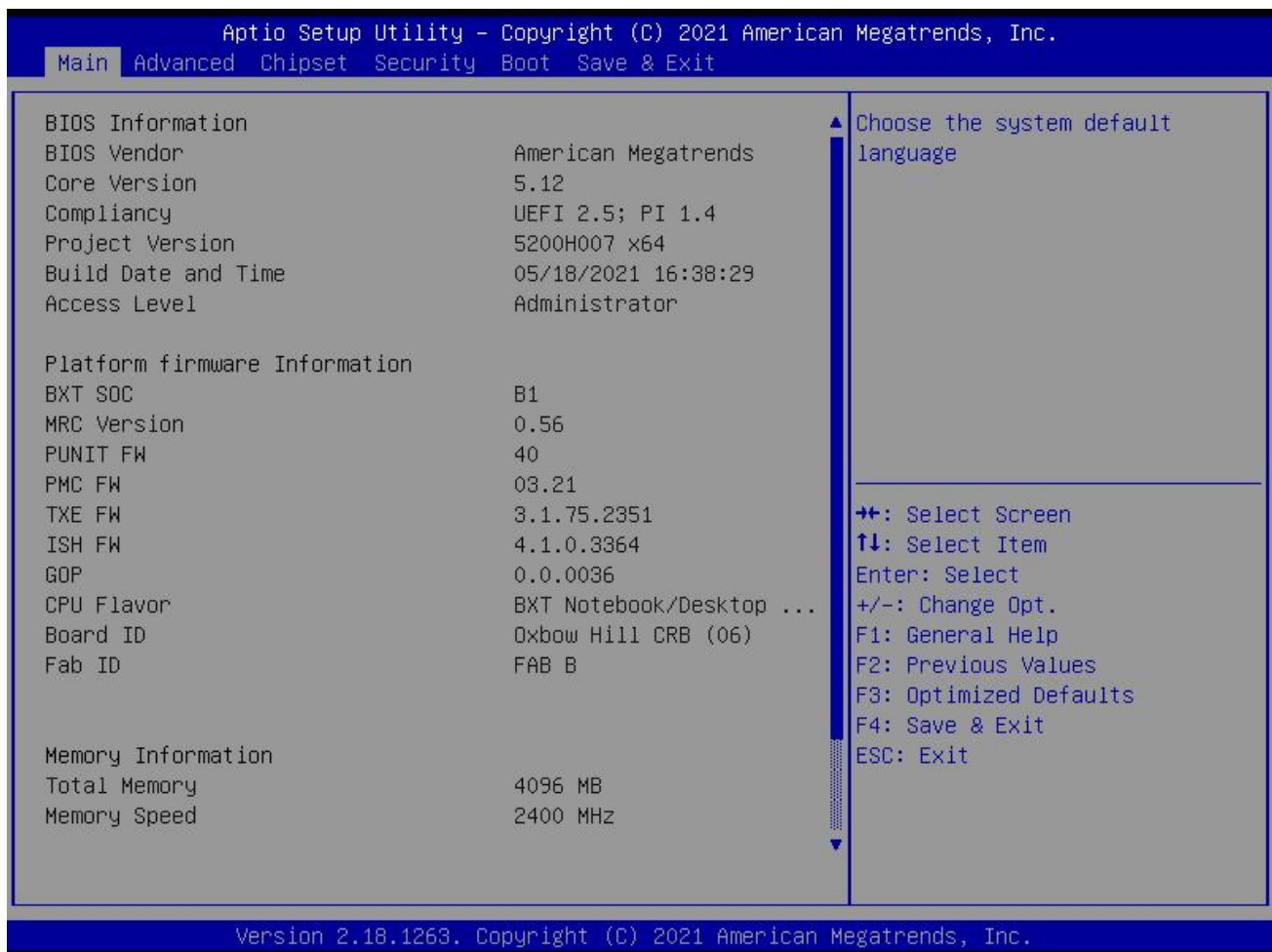
Main menu
