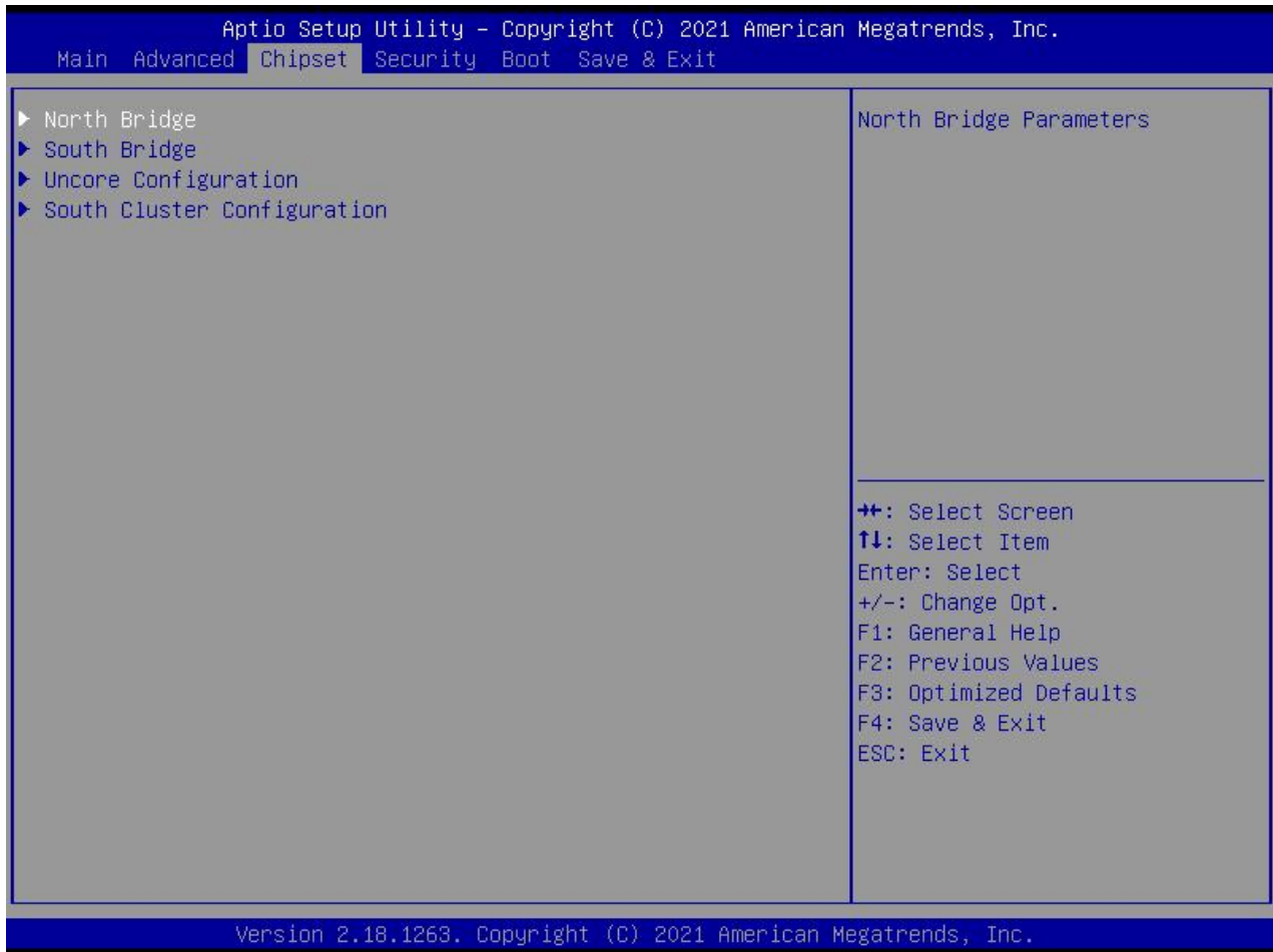
Chipset menu
